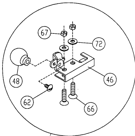
UPPER DOOR LATCH DETAIL 2X SCALE
